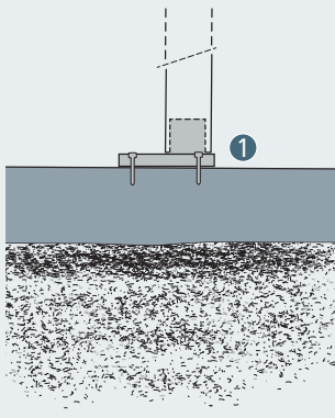
Post fixation on concrete floor slabs
