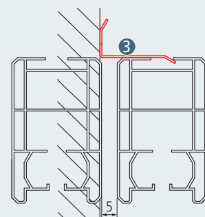
"Small" wall bracket ③, for unit 2 with drive on the right (lateral spacing of 5 mm)
