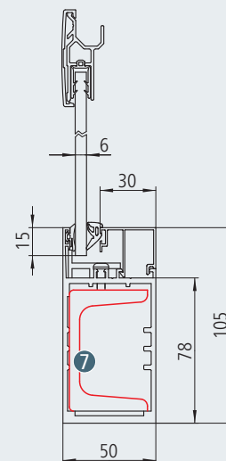
Side element and locking bar with steel reinforcement ⑦
