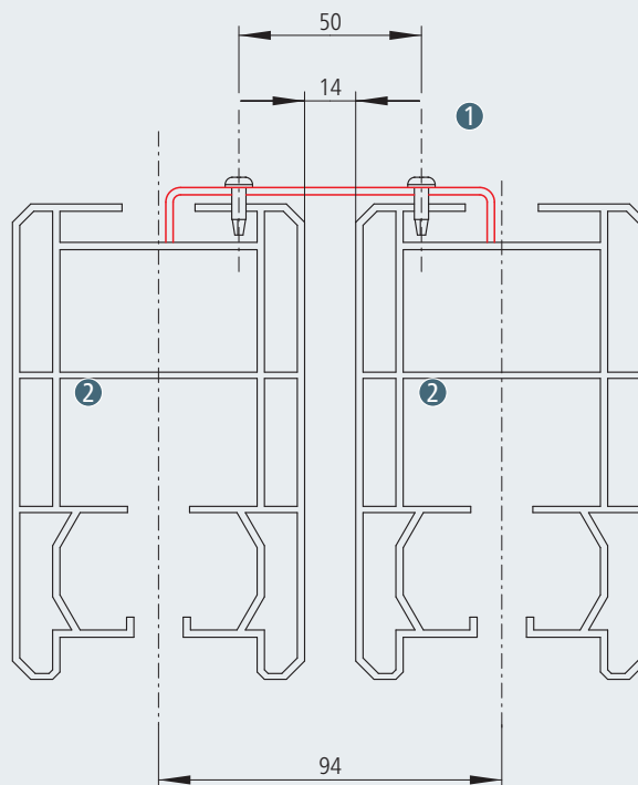
Side channels with coupling panel (profile view)
