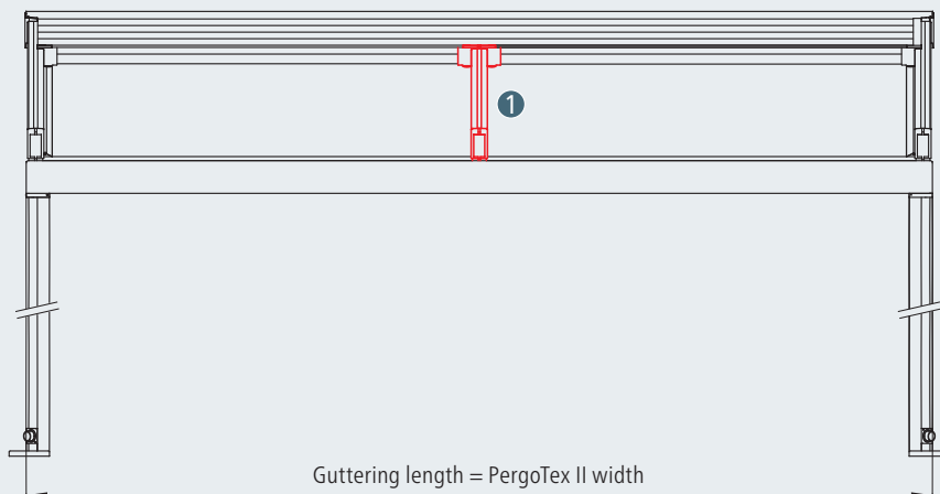
PergoTex II with third side channel
