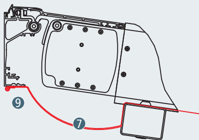
Fabric end > 18° to 25° (for PergoTex II Basic from 0° to 25°)
