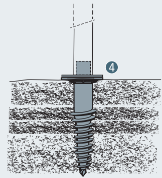
Krinner screw foundation
