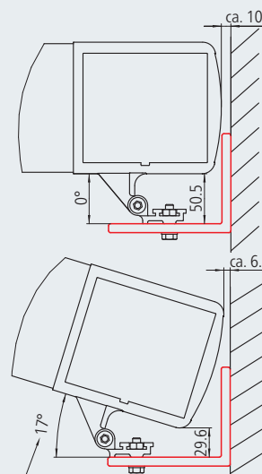
Installation with an angle bracket only possible up to a maximum pitch of 17°
