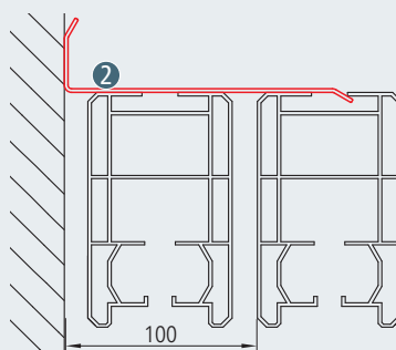
"Large" lateral wall bracket ②, for unit 2 with drive on the left (lateral spacing of 100 mm)
