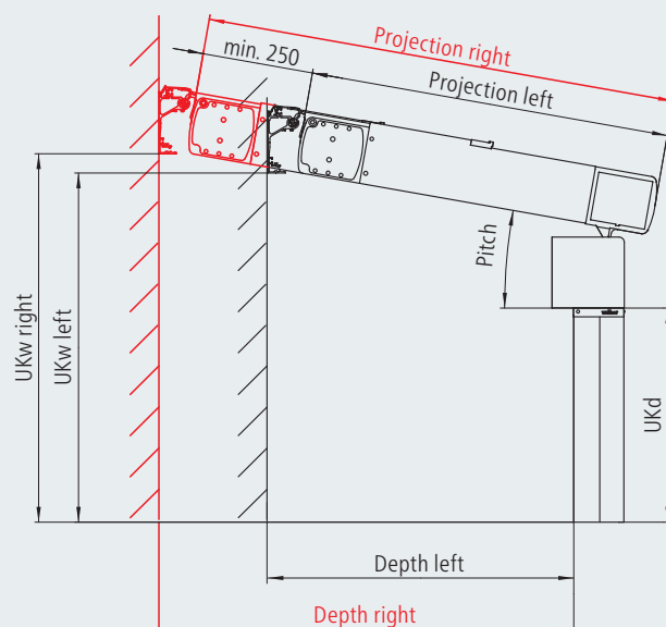
Multi-section unit with offset (profile view)
