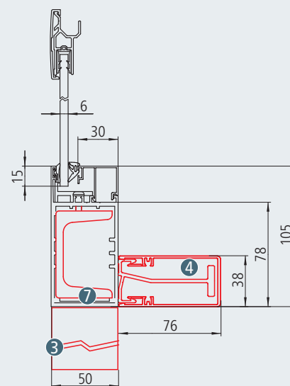
Side element, locking bar with steel reinforcement ⑦, wind support bracket ④, post (rectangular pipe) ③
