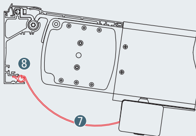
Fabric end from 0° to 18° (not for PergoTex II Basic version)
