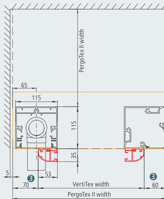
Top view of the VertiTex rail guide on the post of the PergoTex II (limited laterally)
